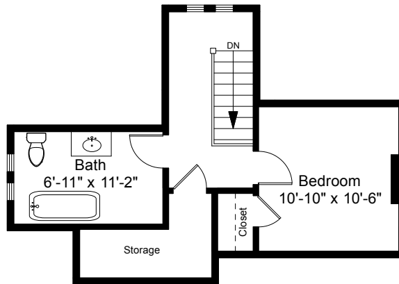
Third Floor Plan Ceiling Height = 7'-2"
