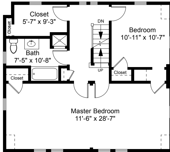
Second Floor Plan Ceiling Height = 7'-8"
