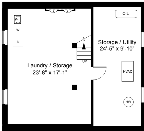
Lower Level Plan Ceiling Height = 7'-0"
